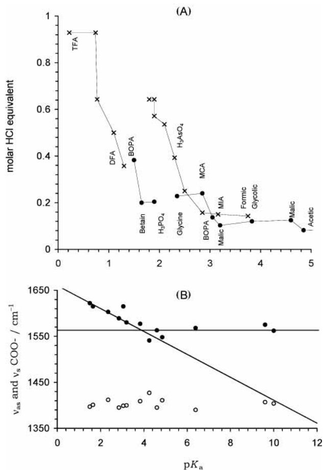
Figure 7. Relationship of pK_a with (A) acidic water (molar HCl equivalent or continuum of absorbance; (●) this work and (x) values from ref 26); (B) \nu_{\text{COO}^-} ((●) asymmetric and (○) symmetric). Slanted straight line comes from the work of Cabaniss and McVey. 37a
