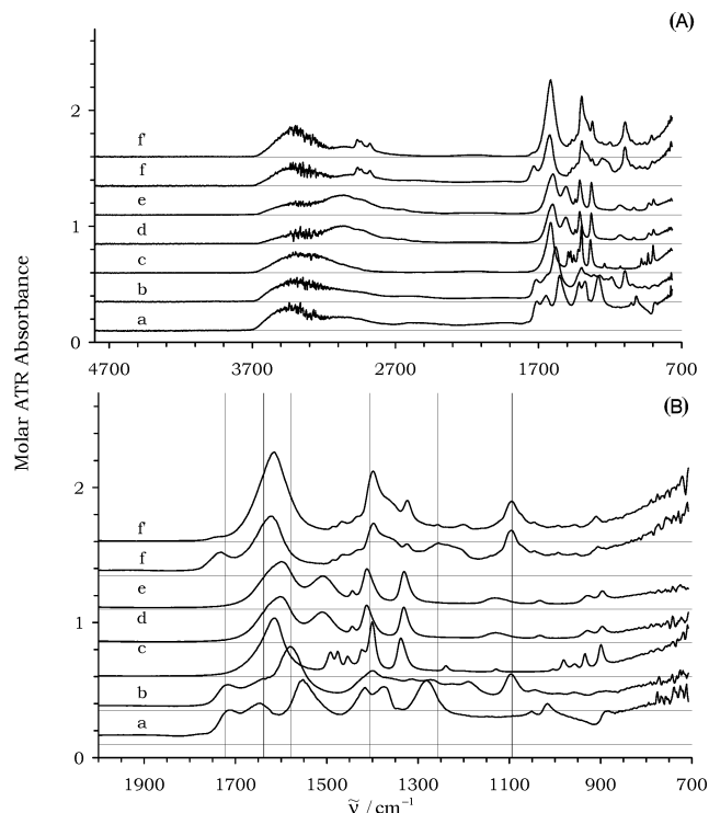
Figure 6. Molar ATR-IR spectra of zwitterionic carboxylic acids ( N^+COO^- ) and special cases: spectrum c, betaine; spectrum d, 1.33 M glycine; spectrum e, 2.66 M glycine; spectrum f, BOPA (one free carboxylic acid group); spectrum f', BOPA (no free carboxylic acid group); spectrum a, sodium aceto-acetate complex; spectrum b, monosodium malate. Panel A shows the complete region, and panel B shows the expanded region. Vertical lines at 1723, 1643, 1579, 1406, 1257, and 1094 cm^{-1} .
